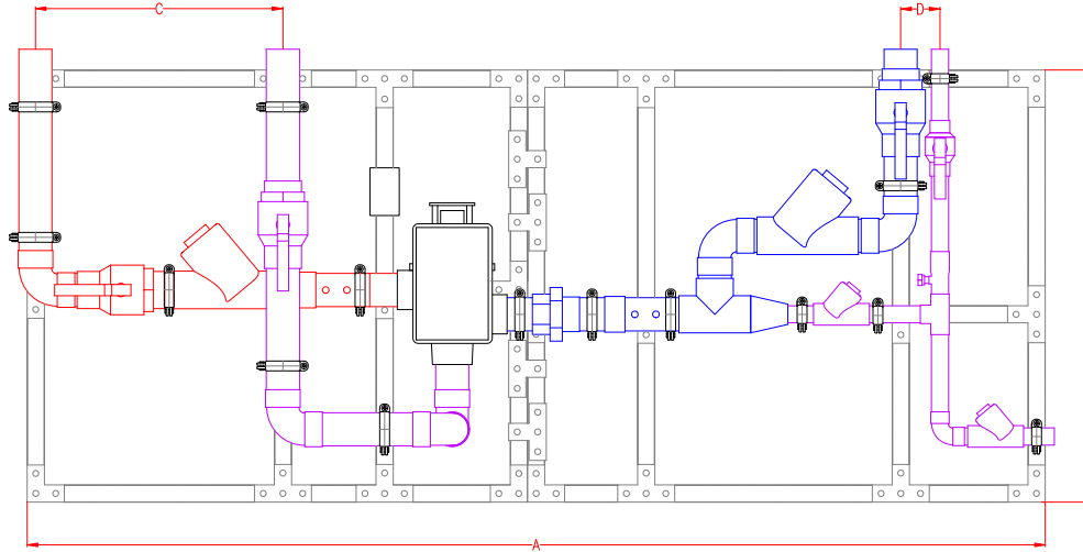
APPROXIMATE DIMENSIONS A = 8'-0" B = 3'-5" C = 1'-11" D = 4" *Image not to scale*
